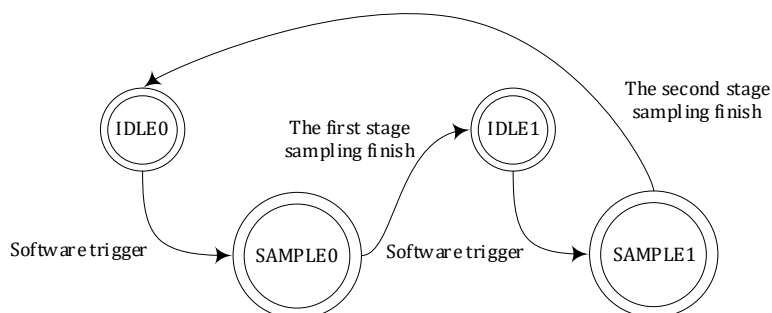
Fig. 10-5 State Transition Diagram of ADC Two-round Sampling
