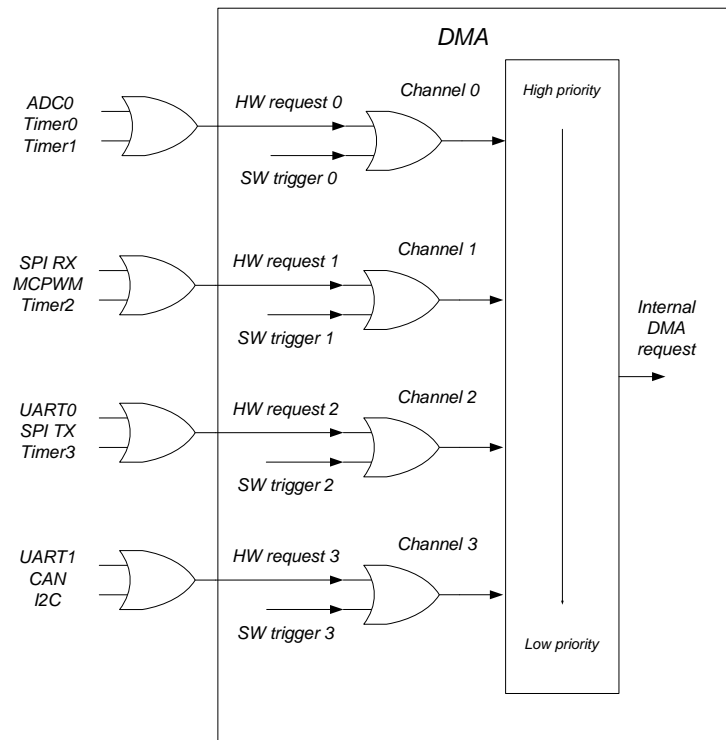
Fig. 7-3 DMA Channel Priority
