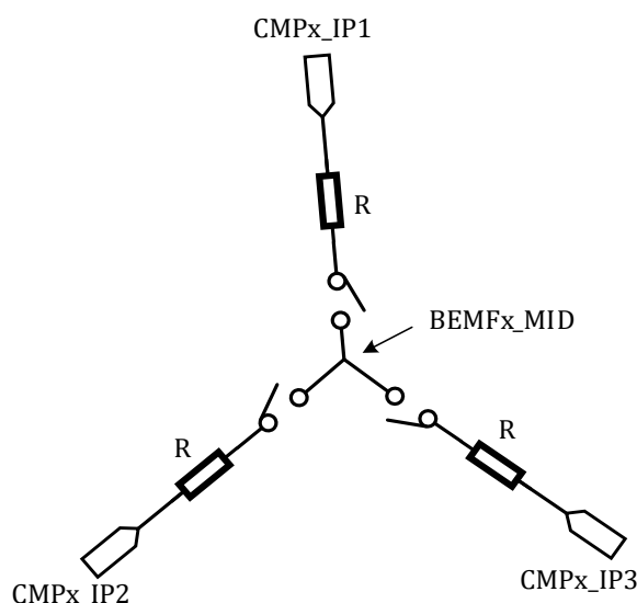
Fig. 18-2 BEMF_MID Signal
