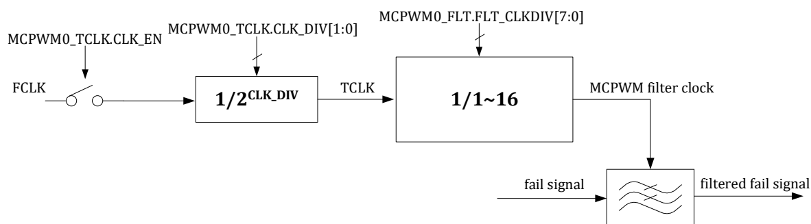
Figure 14-6 MCPWM Fail Signal Filter Clock Generation Logic
