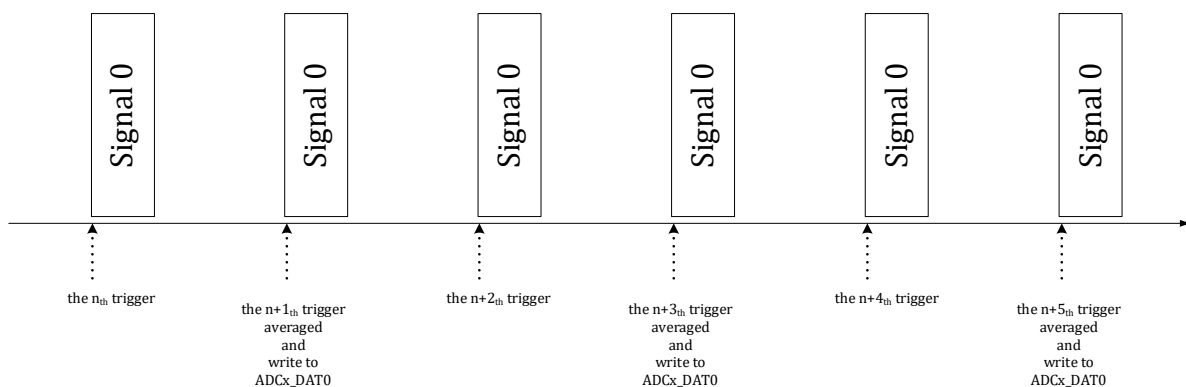
Figure 12-5 Oversampling Conversion Timing Example 2
