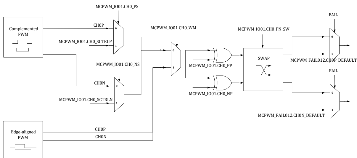
Figure14-7 IO Driver Module Data Flow Diagram
