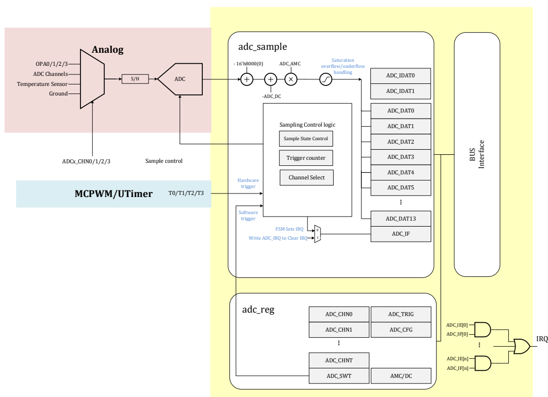
Figure 12-1 ADC Acquisition Module Functional Block Diagram
