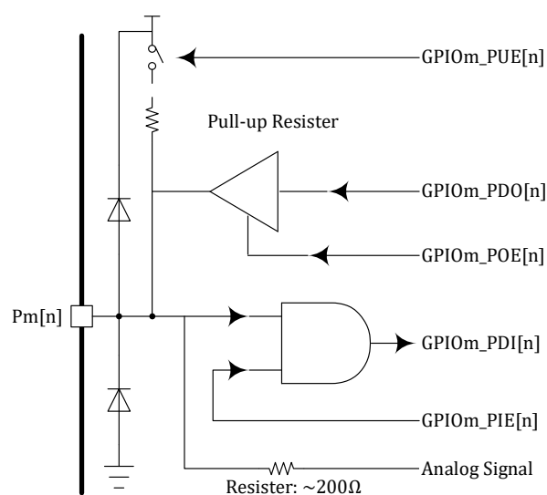
Figure15-1 GPIO Functional Block Diagram
