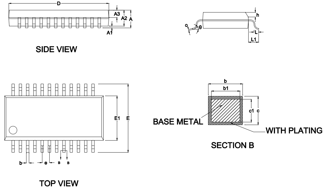
Fig.4-6 LKS32MC077MBS8 Package Diagram
