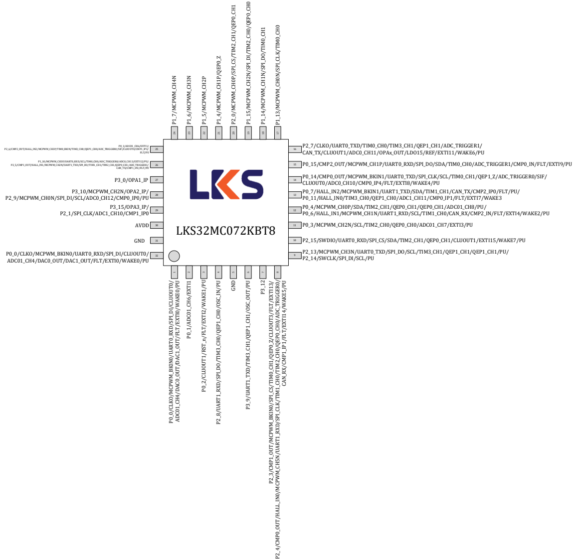
Fig.3-5 LKS32MC072KBT8 Pin Assignment
