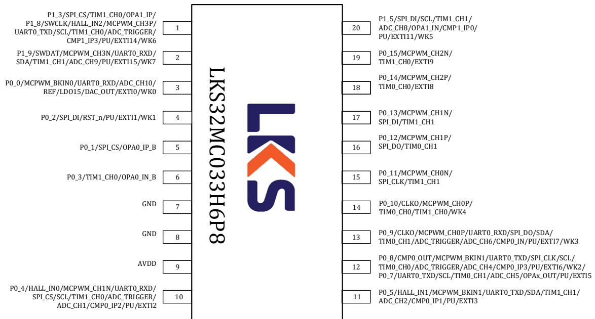
Figure 3-2 LKS32MC033H6P8 Pin Assignment Diagram
