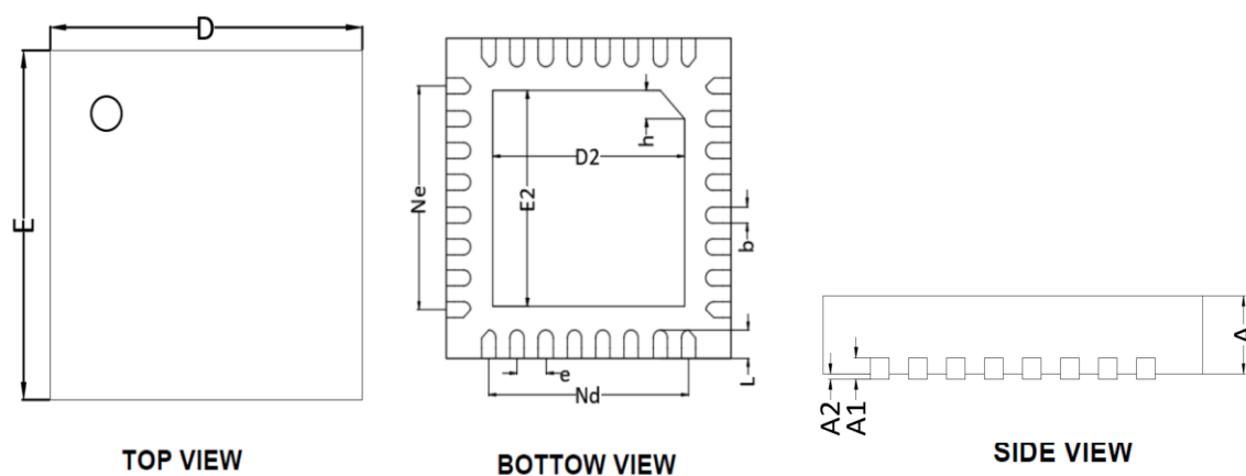
Figure 4-4 LKS32MC0342FLK6Q8C/LKS32MC034FLNK6Q8C/LKS32MC034F2LNK6Q8C Packaging
