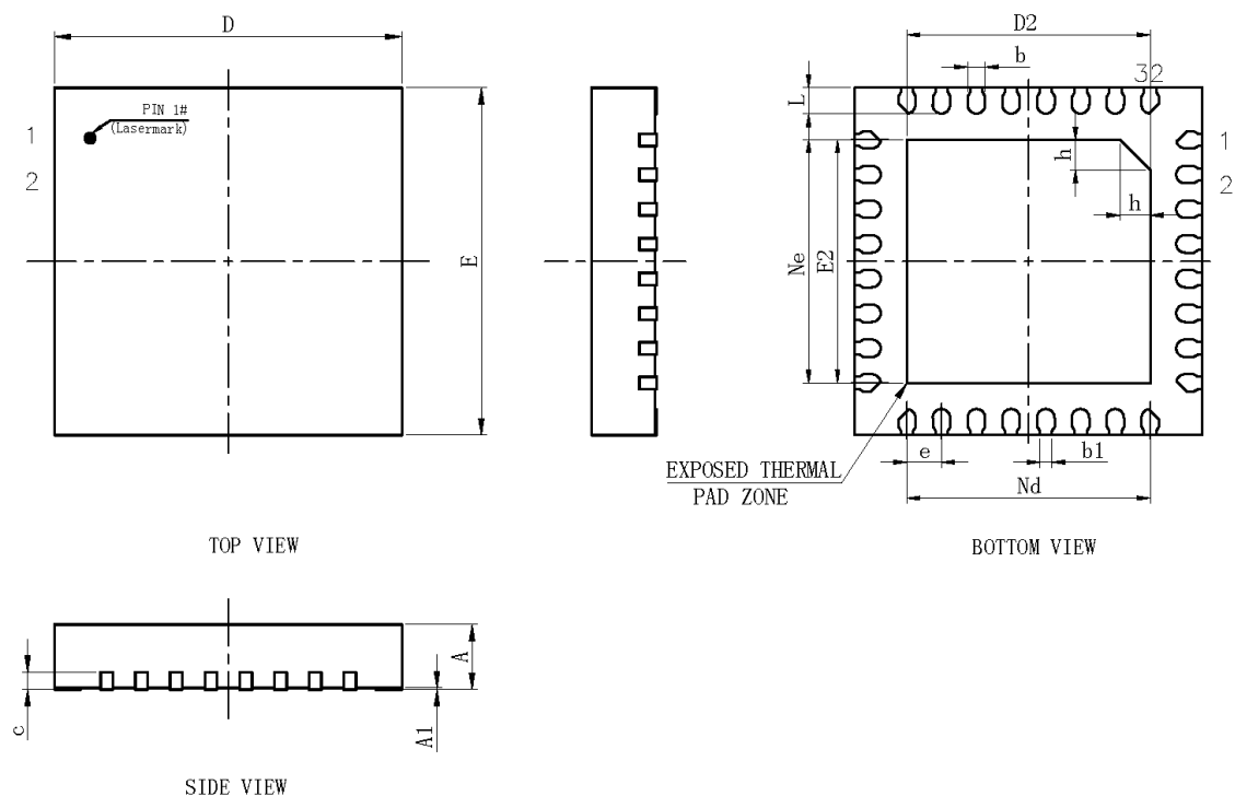
图 4-5 LKS32MC039DK6Q8B(C)/ LKS32MC039PL3K6Q8C/ LKS32MC039D2K6Q8C 封装图示
