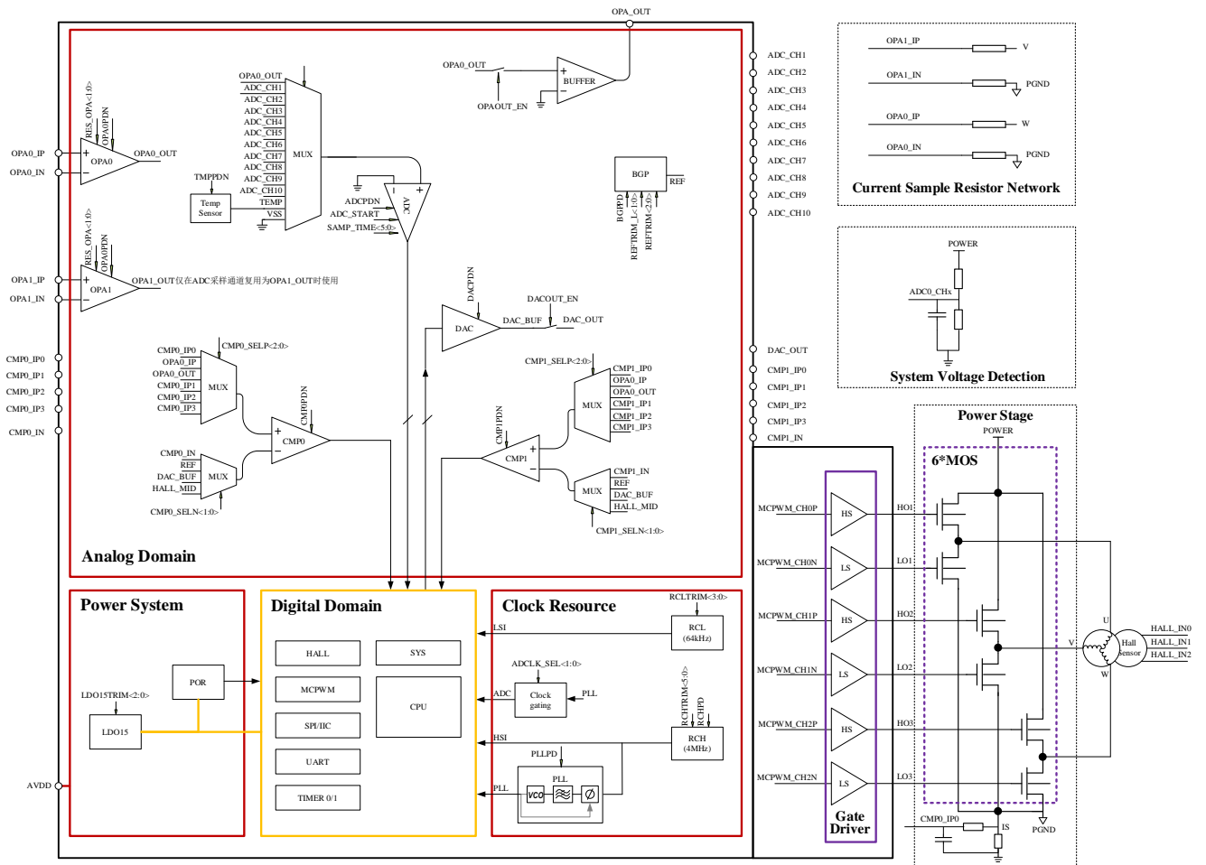
Figure 1-2 Simplified Schematic Diagram of the LKS32AT037PXL5M6Q9 Vector Sinusoidal Control System
